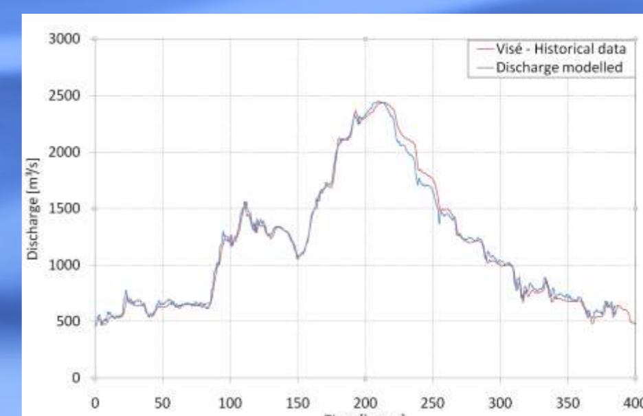
Comparison of the historical and modelled discharge in Lixhe
